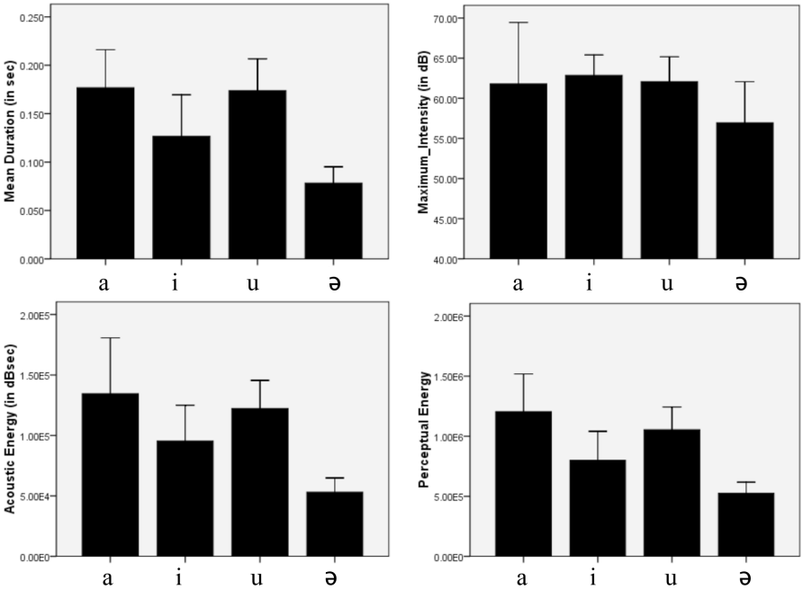
Figure 11. Duration (top left), maximum intensity (top right), acoustic energy (bottom left), and perceptual energy (bottom right) values averaged across one male K w ak w ala speaker. Whiskers indicate one standard deviation from the mean.
