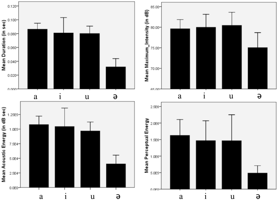
Figure 5. Duration (top left), maximum intensity (top right), acoustic energy (bottom left), and perceptual energy (bottom right) values averaged across four Be-semah speakers. Whiskers indicate one standard deviation from the mean.
